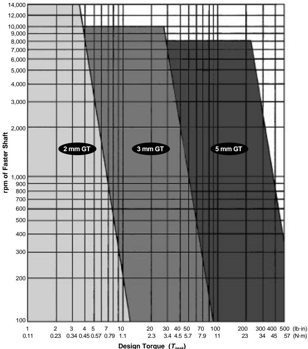
Fig. 41 GT Belt Selection Guide
