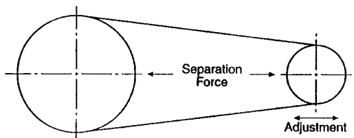
Fig. 21 Shaft Separation Method
