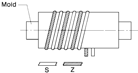
Fig. 18 "S" and "Z" Cord Lay of the Mold
