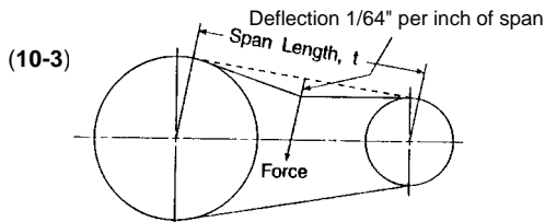
Fig. 20 Force/Deflection Method
